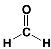
formaldehyde
