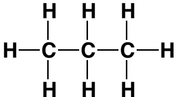
propane
