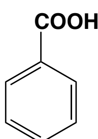
benzoic acid
