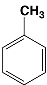
toluene
