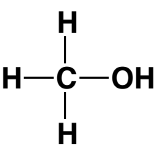
methanol
