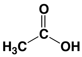
acetic acid
