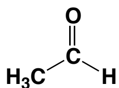
acetaldehyde
