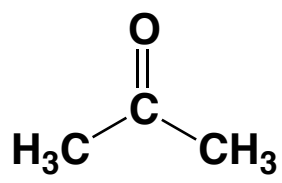
acetone
