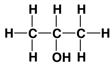
isopropyl alcohol
