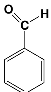
benzaldehyde
