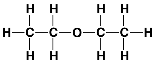
ethyl ether
