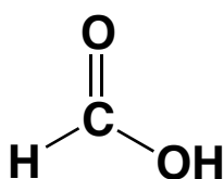
formic acid
