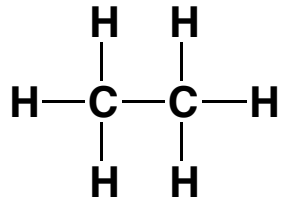
ethane
