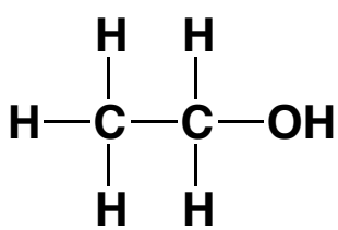
ethanol
